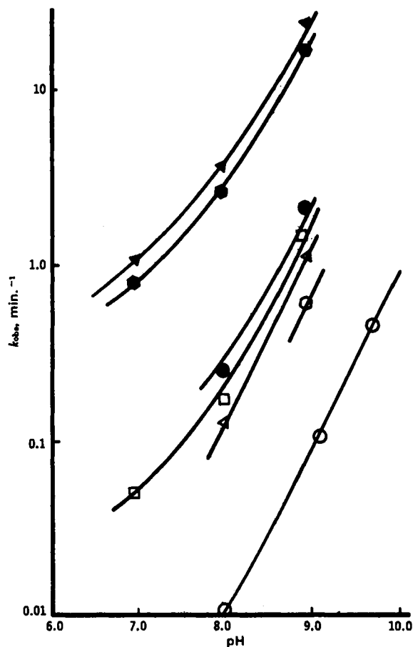
Figure 1—Plot of \log k_{obs} versus pH for hydrolysis of N -acyl phthalimides. Key: \circ , R = N(CH_3)_2 ; \circ , R = \text{morpholino} ; \Delta , R = C_2H_5 ; \square , R = C_2H_5O ; \bullet , R = CH_3 ; \circ , R = CH_2Br ; and \blacktriangle , R = CH_2Cl . (For definition of R , see Scheme I.) (*Unpublished data, T. Higuchi and F. Kametani.)
